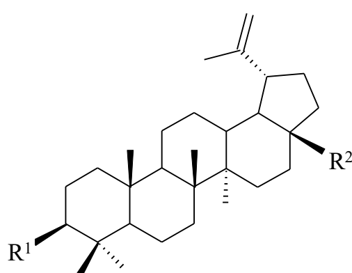
Figure 1. Chemical structures of pentacyclic triterpenes.
